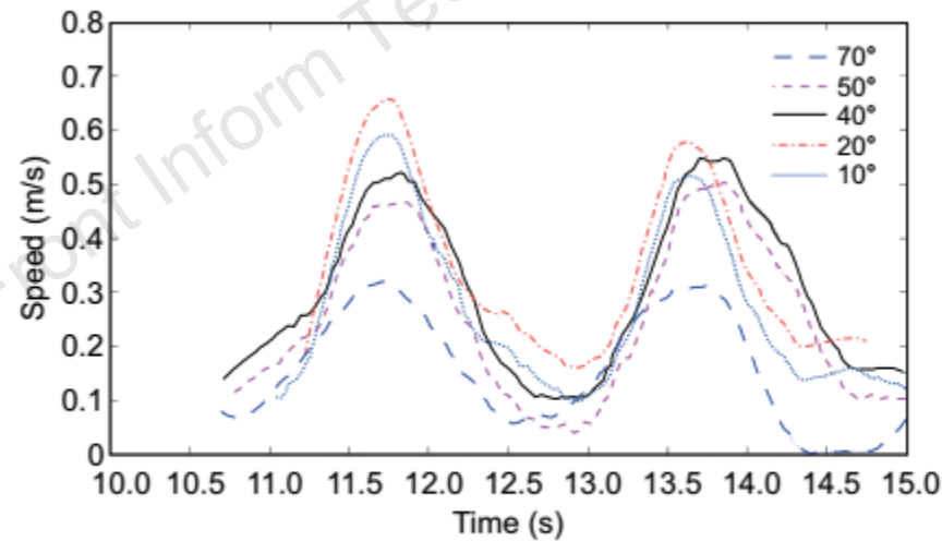
Fig. 11 Forward speeds under different angles of attack
