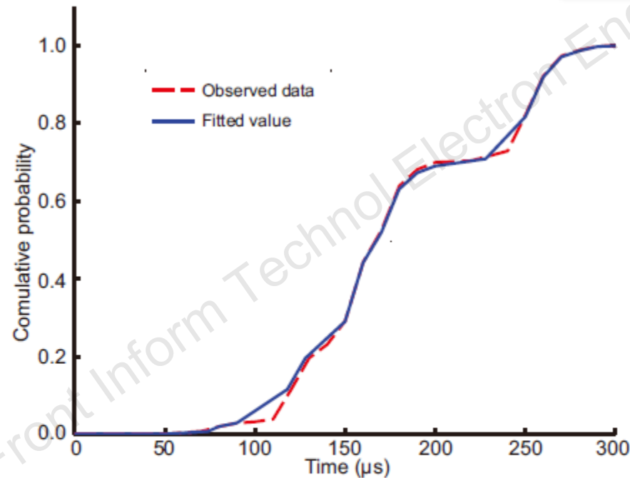
Fig. 15 Delay time comparison between the fitted value and practical observation for M_{N2} in case study 2 (root mean square error: 0.0140; maximum absolute error: 0.0423)
