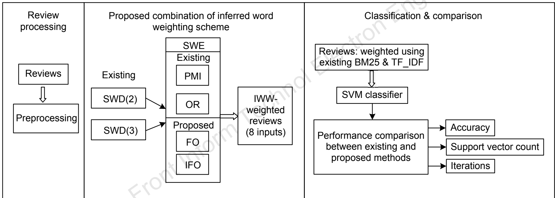
Workflow of the proposed weighting and classification
