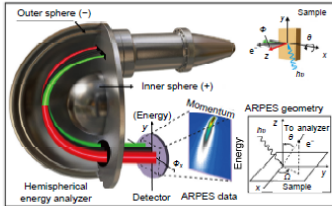
Fig. 28 Principle of a modern ARPES with a hemispherical electron energy analyzer (reprinted from Zhou et al. (2018), Copyright 2018, with permission from the IOP Publishing Ltd.)
