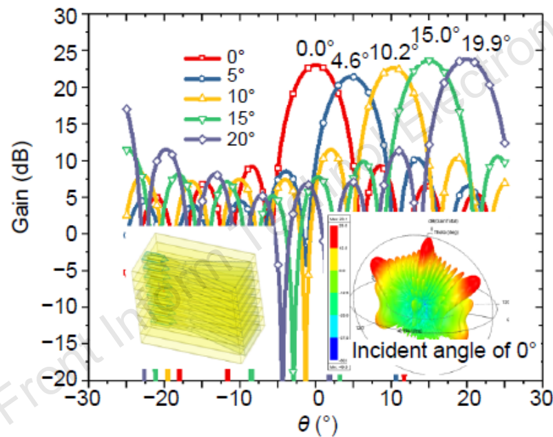
Fig. 10 Scanning radiation pattern of the retrodirective array versus different incident angles
