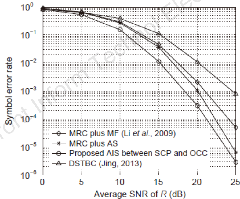
Fig. 5 Curves of the symbol error rate versus the average \text{SNR}_R with 16-QAM ( \text{SNR}_D = \text{SNR}_R )
