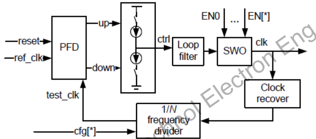
Fig. 7 SWO based PLL architecture
