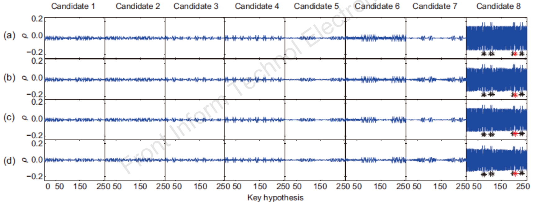
Fig. 19 Results of partial-CPA 3 toward \varphi_0 : (a) case A; (b) case B; (c) case C; (d) case D
