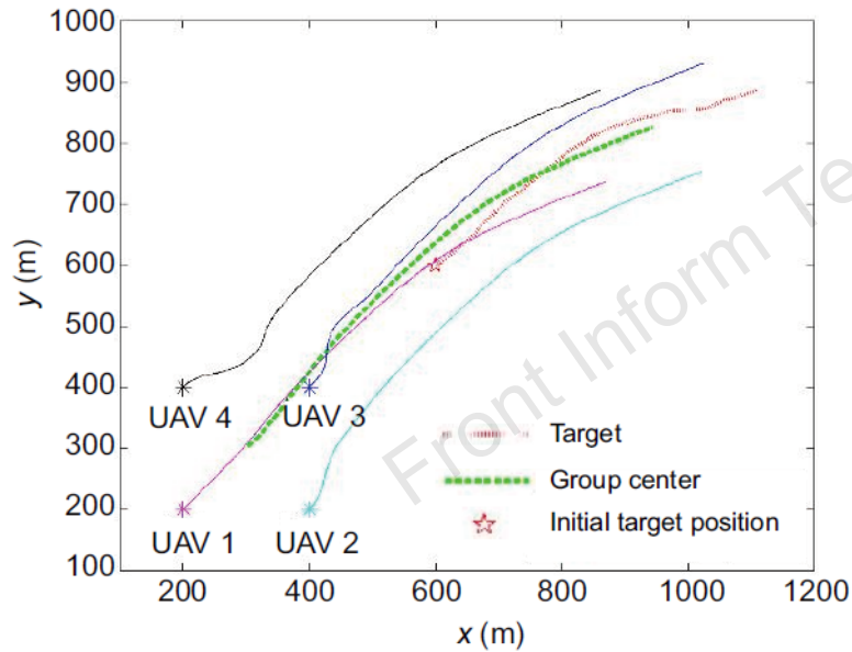
Fig. 1 Trajectories of the target and UAVs in Example 1
