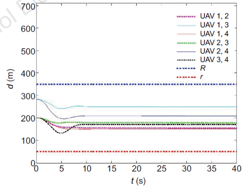
Fig. 2 Inter-UAV distances in Example 1
