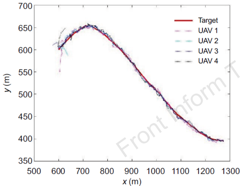
Fig. 7 Target trajectory and estimated trajectories of the four UAVs in Example 2
