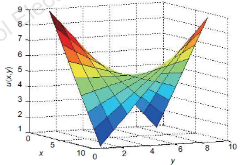
Fig. 2 Plot of the proposed solution for case 1 (Laplace equation with Dirichlet boundary conditions)
