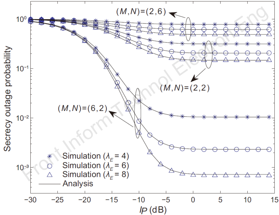
Fig. 2 Secrecy outage probability versus I_P for \lambda_D = 2 , \lambda_P = 3 , N_0 = 1 , P_S = 1 dB, and C_{th} = 0.1\text{bit}/(\text{s}\cdot\text{Hz})
