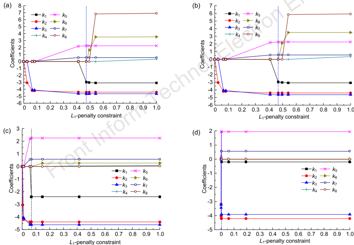
Fig. 3 The coefficient selection paths of the subthreshold current under different conditions: (a) \lambda_1=1e-13 , \min(AIC)=63.0989 ; (b) \lambda_1=1e-5 , \min(AIC)=63.0994 ; (c) \lambda_1=1e-2 , \min(AIC)=63.6353 ; (d) \lambda_1=0.5 , \min(AIC)=84.1606
