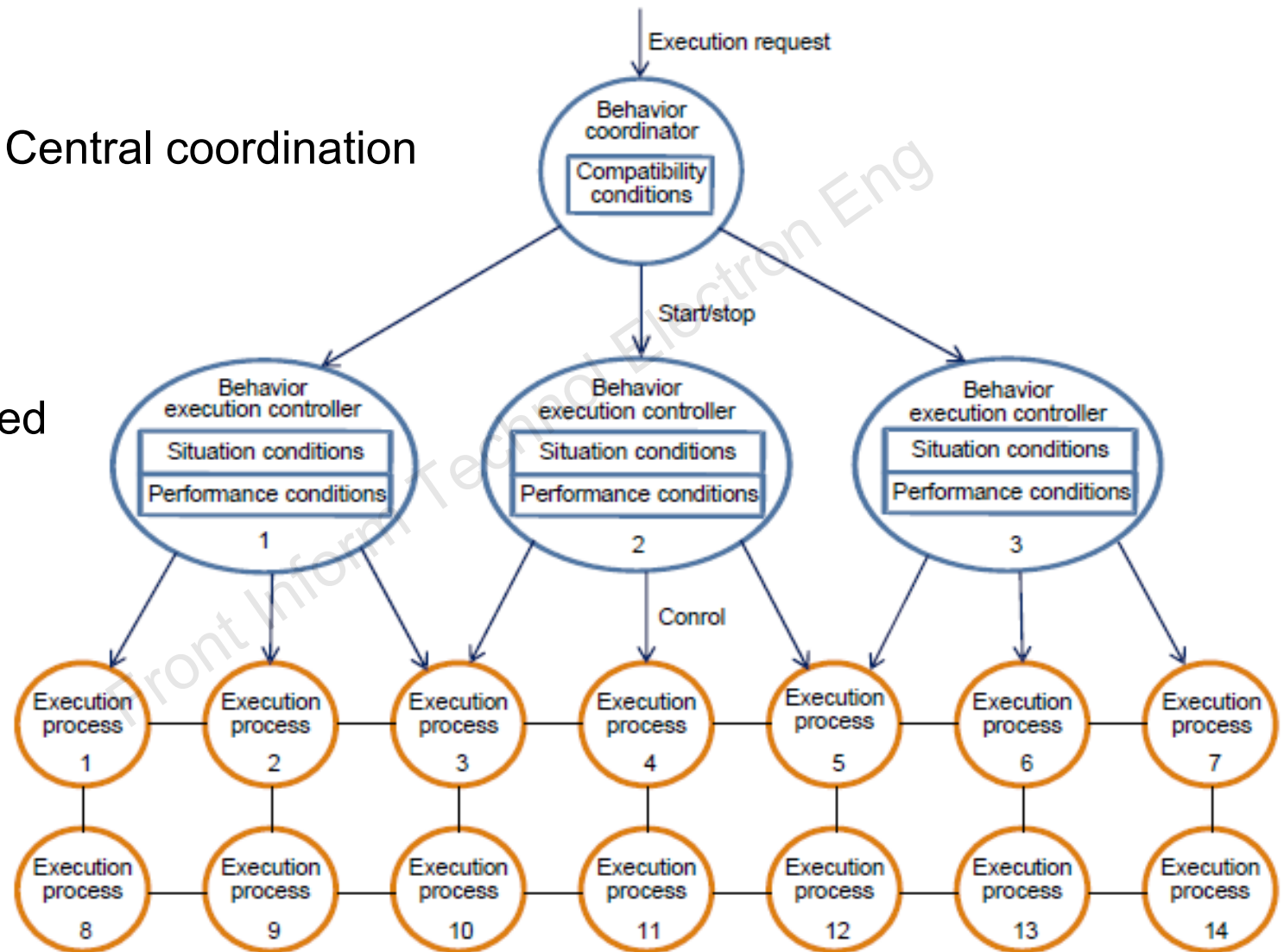
Fig. 3 Distributed scheme for execution control
