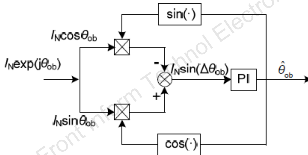
Fig. 7 Block diagram for a position observer
