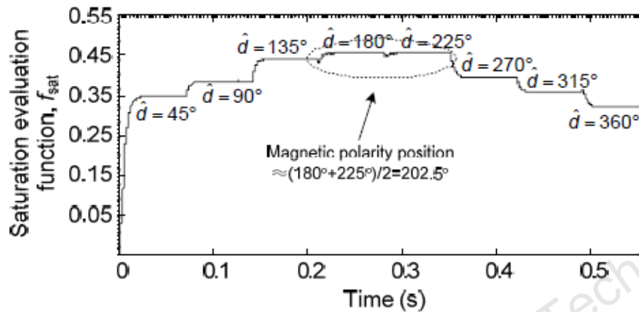
Fig. 11 Simulation process for identification of magnetic polarity
