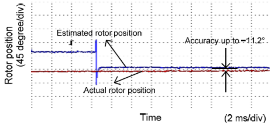
Fig. 18 Experimental results for the position observer
