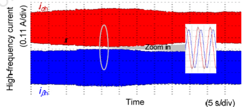
Fig. 15 Extracted 500 Hz current responses in the \alpha - \beta frame
