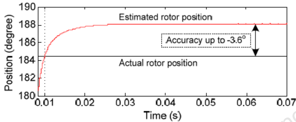
Fig. 13 Simulation performance of the position observer
