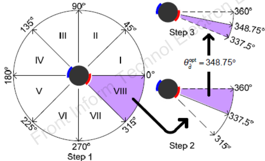
Fig. 6 Saturation-based magnetic polarity identification
