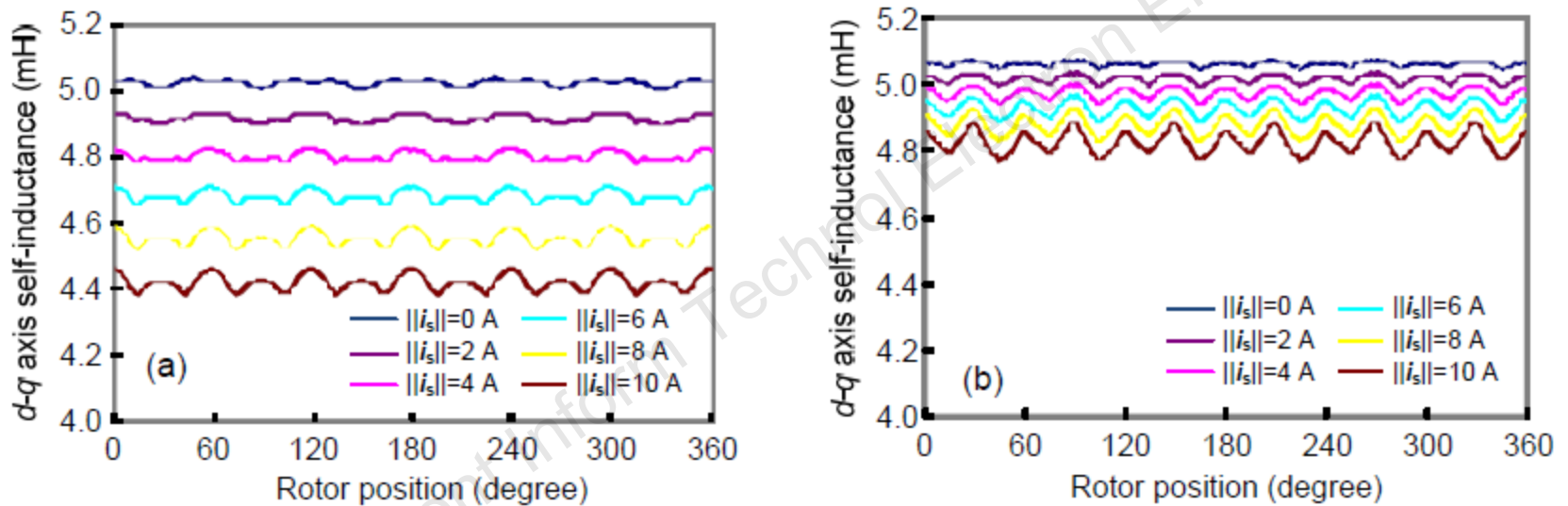
Fig. 3 Inductance-position characteristics: (a) L_{qq} -position; (b) L_{dd} -position
