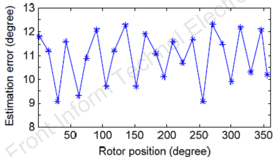
Fig. 19 Distribution of the estimation error versus rotor position
