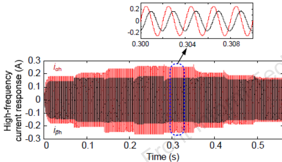
Fig. 10 Simulation results for extracting 500 Hz currents
