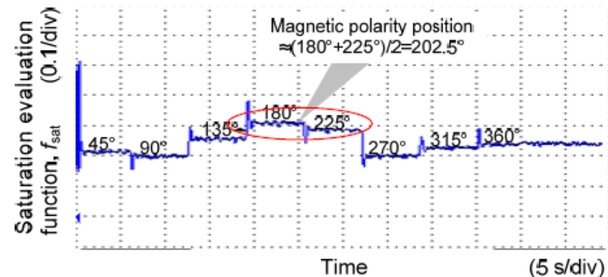
Fig. 16 Experimental process for identification of magnetic polarity
