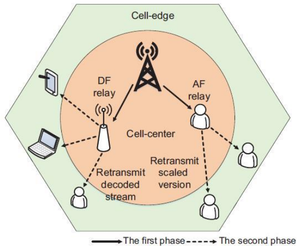
Relay NOMA
