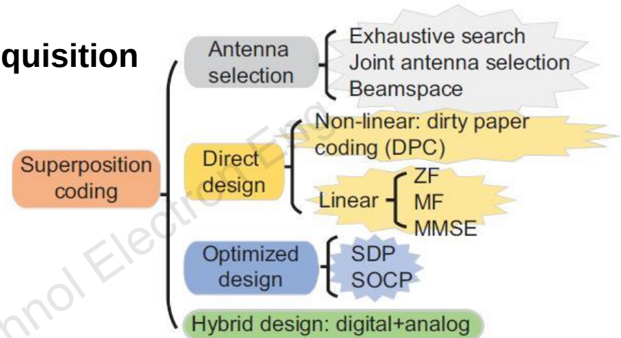
The illustration of superposition coding schemes
