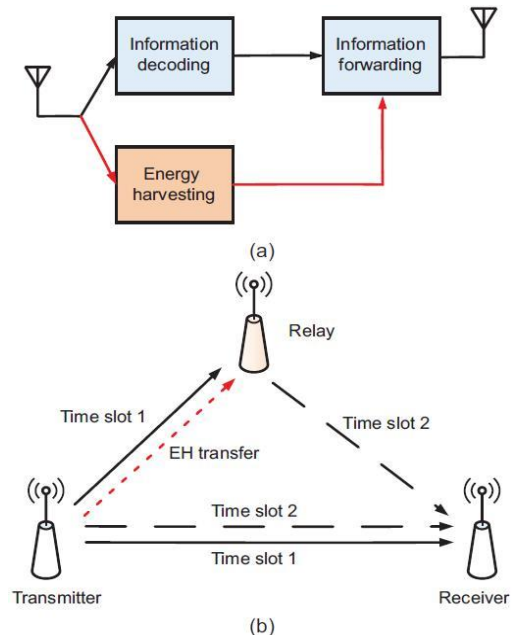
Simultaneous wireless information and power transfer in NOMA
