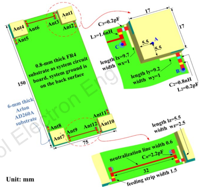
Fig. 6 Geometry of the 12-element MIMO array
