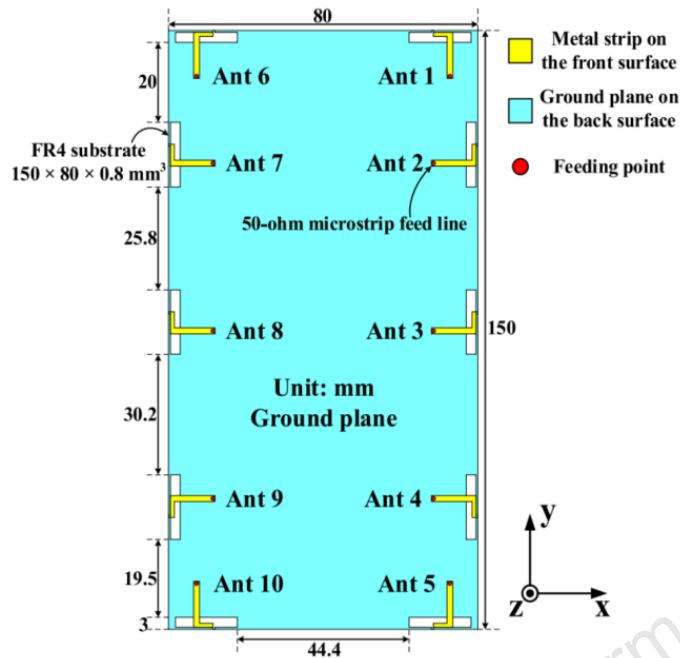
Fig. 5 Geometry of the ten-element MIMO array
