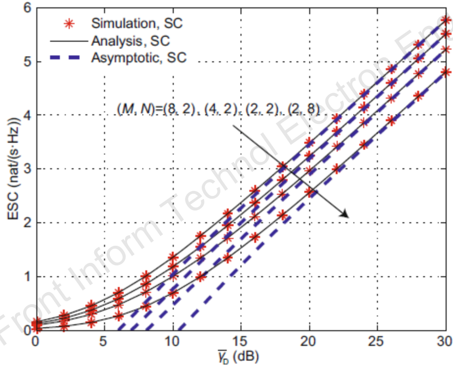
Fig. 5 ESC vs. \bar{\gamma}_D of SC with outdated CSI for \bar{\gamma}_E = 5 \text{ dB} , \rho_D = 0.5 , \rho_E = 0.6 , N_0 = 1 , and P_S = 3 \text{ dB}
