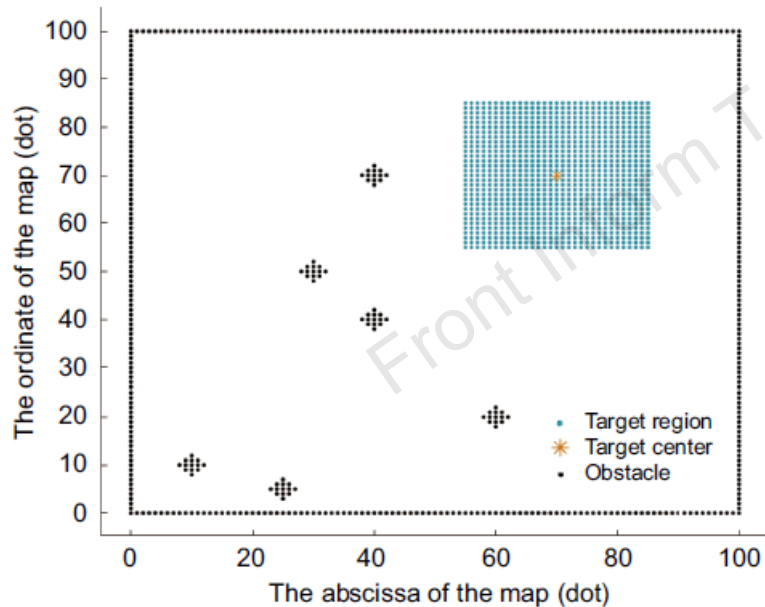
Fig. 1 Scenario model of the navigation algorithm (100 × 100). The scenario model of the whole task space is P \times Q
