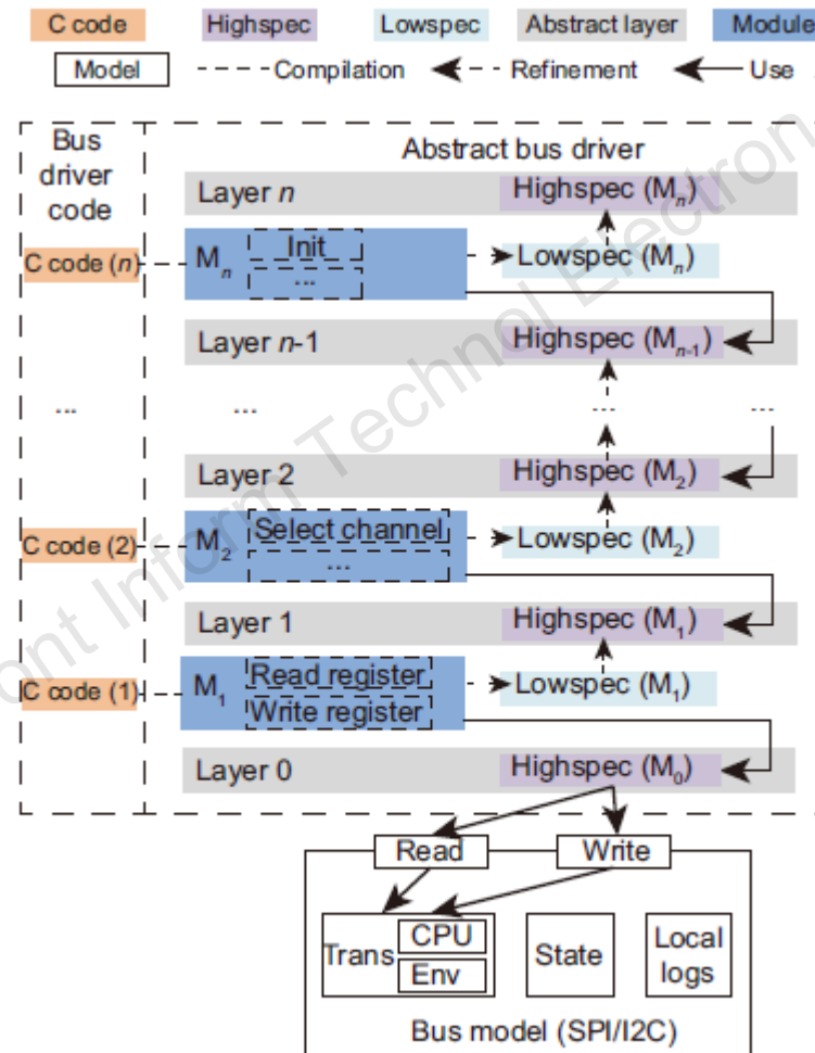
Fig. 2 Driver verification structure
