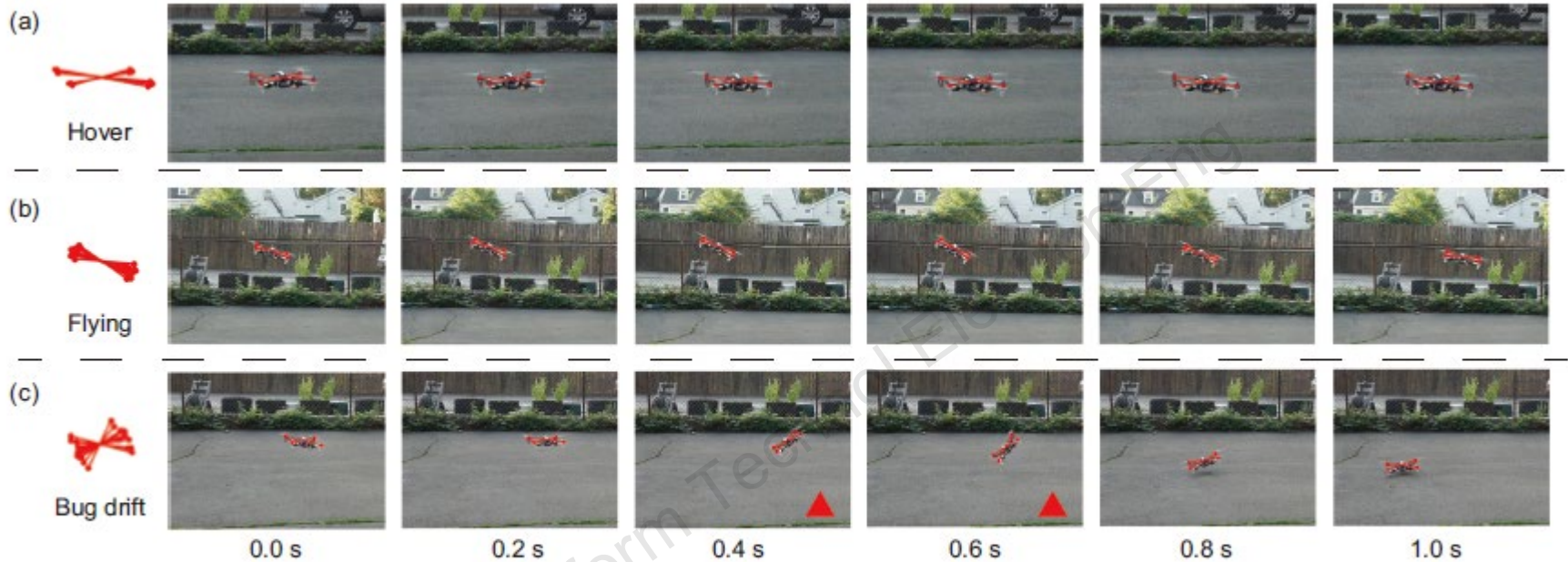
Fig. 13 Empirical comparison between systems with ((a) and (b)) or without (c) a verified SPI bus driver
