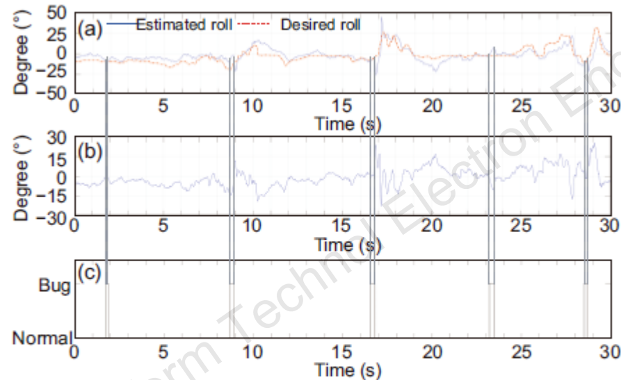
Fig. 9 Roll angle response of drone with an unverified SPI bus driver: (a) roll angle; (b) roll angle error; (c) SPI bus bug
