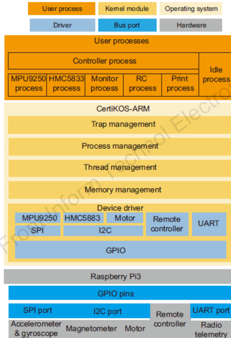
Fig. 1 Overall software architecture
