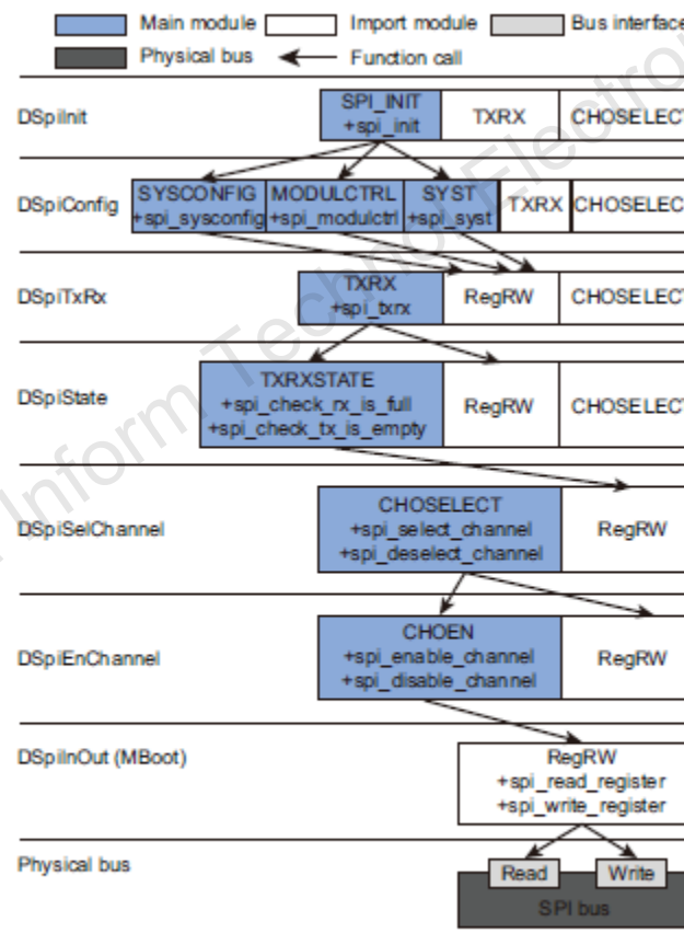
Fig. 3 Layering structure of the SPI bus driver
