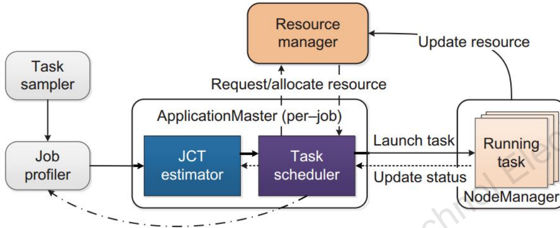
A architecture overview of our proposed scheduler
