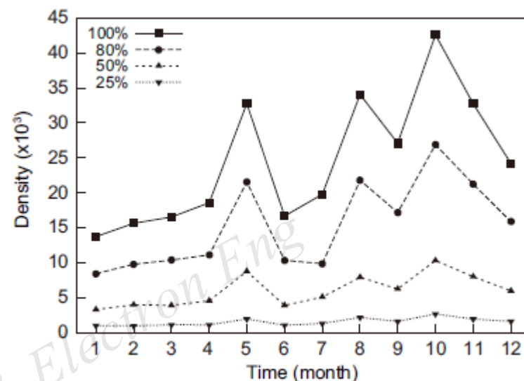
Fig. 12 The density at different network sizes
