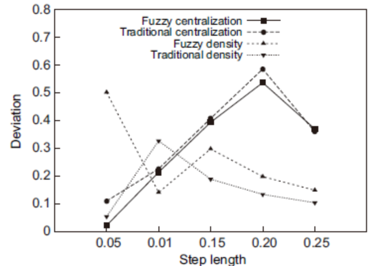
Fig. 8 The difference in deviation between the traditional network and the fuzzy network (10-day call)
