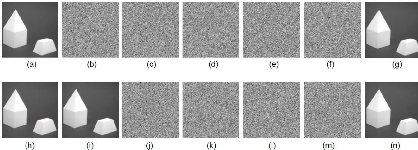
Fig. 9 More experimental results of the proposed (k, n) threshold ISS scheme with bidirectional shadow image authentication without pixel expansion, where k = 3 and n = 4 : (a) grayscale secret image S ; (b–e) grayscale shadow images SC_1 , SC_2 , SC_3 , and SC_4 ; (f–i) grayscale secret image S' decoded with two or more shadow images; (j) fake shadow image SC'_1 ; (k–n) grayscale secret image S' decoded with SC'_1 and the other one or more shadow images
