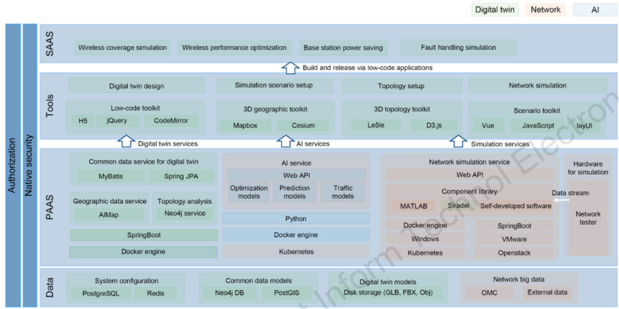
Implementation of the DTN prototype
