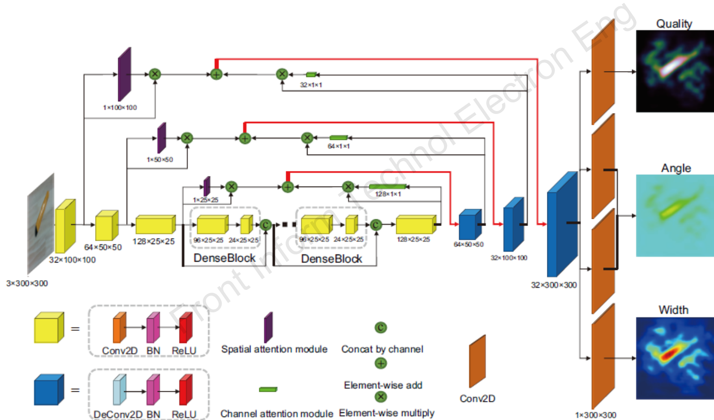
Fig. 3 Model architecture
