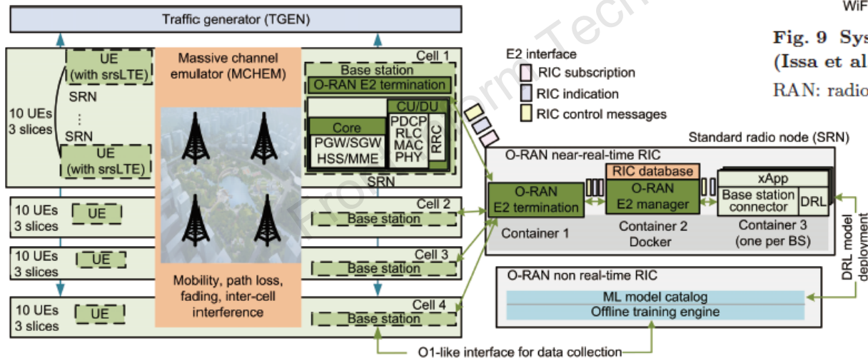
Fig. 10 O-RAN integration in Colosseum (Bonati et al., 2020)
