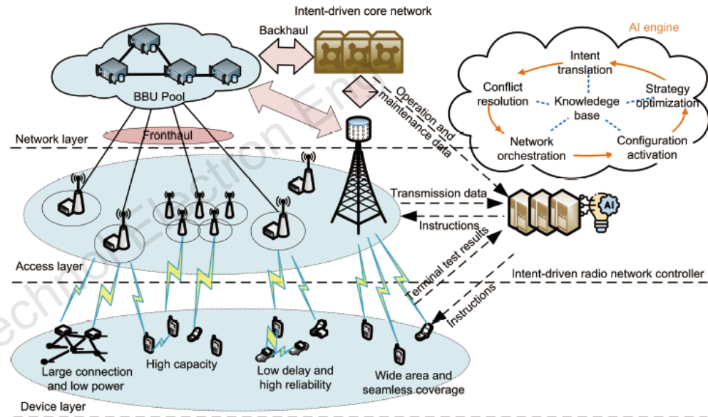
Fig. 4 Intent-driven radio access network architecture (Zhou et al., 2020)
