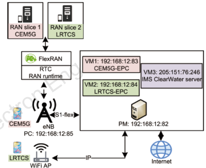
Fig. 9 System structure of the experimental scenario (Issa et al., 2019)
