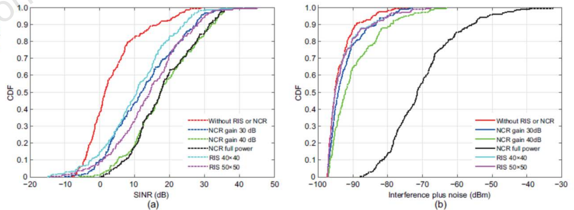
Fig. 8 SINR performance comparison of different repeater-assisted systems, where the carrier frequency is 26 GHz: (a) CDFs of the SINR; (b) CDFs of the noise and interference (SINR: signal-to-interference-and-noise ratio; CDF: cumulative distribution function; RIS: reconfigurable intelligent surface; NCR: network-controlled repeater)
