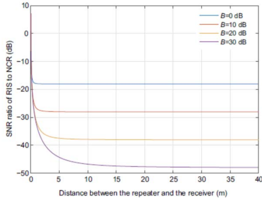
Fig. 3 SNR ratio of RIS to NCR with different NCR amplitudes B (SNR: signal-to-noise ratio; RIS: reconfigurable intelligent surface; NCR: network-controlled repeater). References to color refer to the online version of this figure
