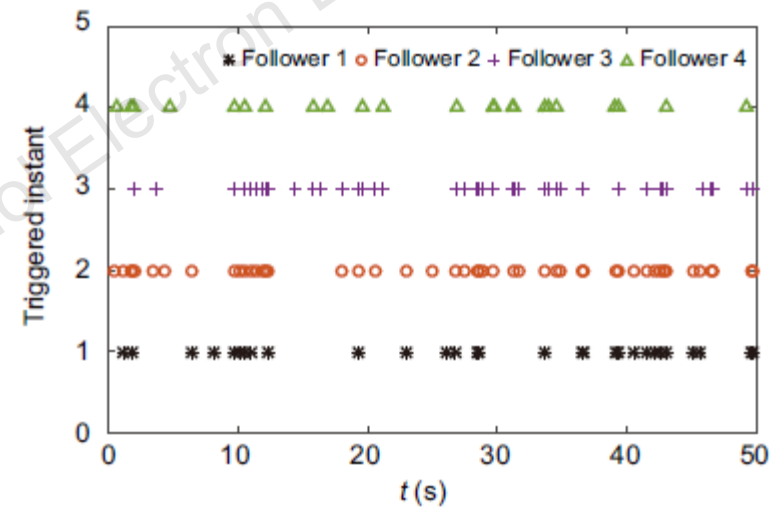
Fig. 5 Triggered instants of the followers under the event-triggered scheme
