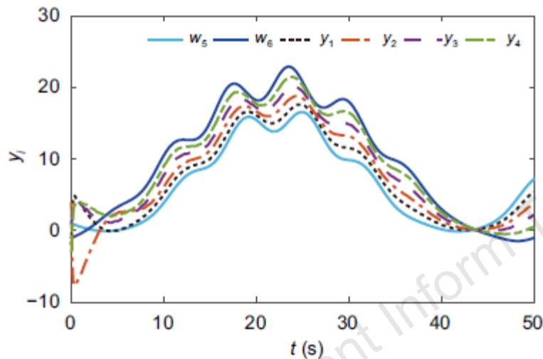
Fig. 3 Outputs of the followers under the event-triggered scheme
