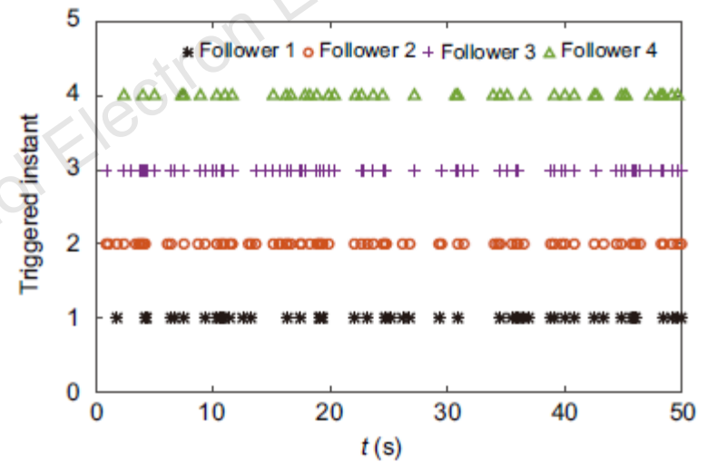
Fig. 9 Triggered instants of the followers under the self-triggered scheme
