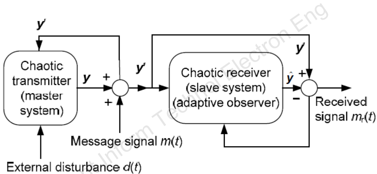
Fig. 5 Block diagram of secure communications using chaotic systems (adapted from Liao and Tsai (2000))
