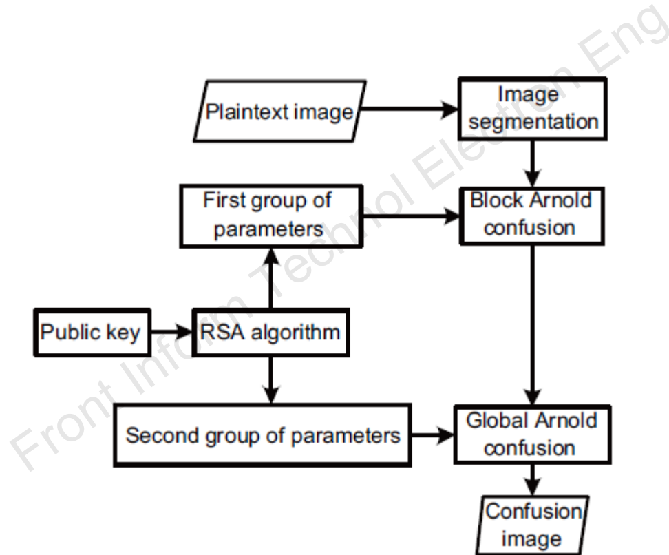
Fig. 2 Asymmetric image confusion algorithm
