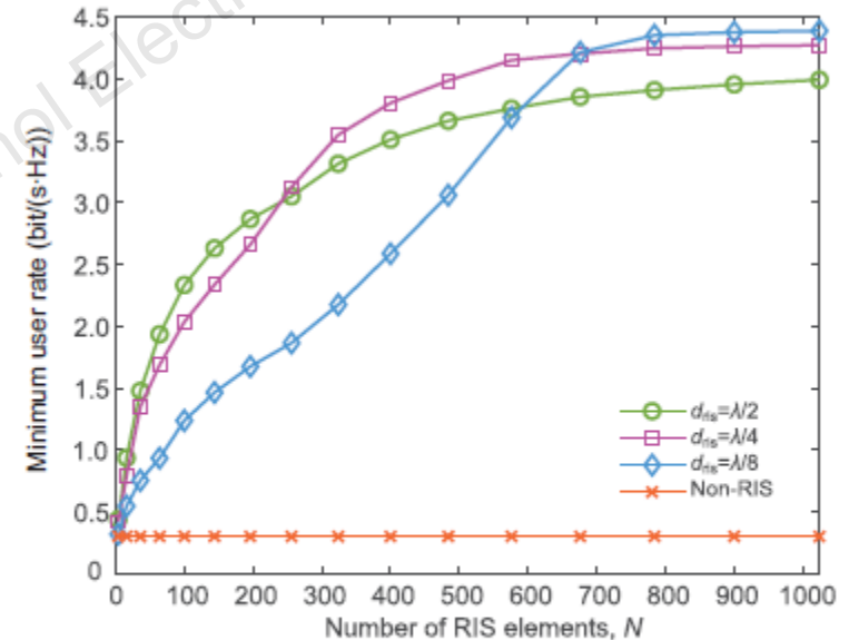
Fig. 9 Max-min achievable rate versus N for different values of the RIS element spacing d_{\text{ris}} (RIS: reconfigurable intelligent surface)
