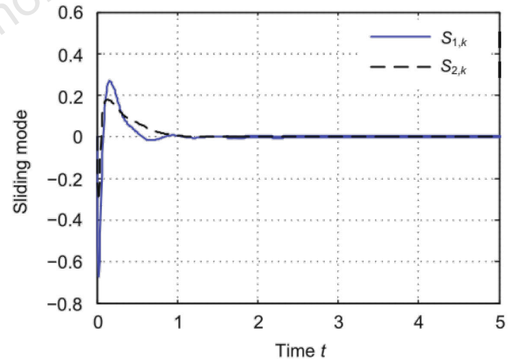
Fig. 12 Sliding mode curves: S_{1,k} and S_{2,k} (sampling time 0.01 s)
