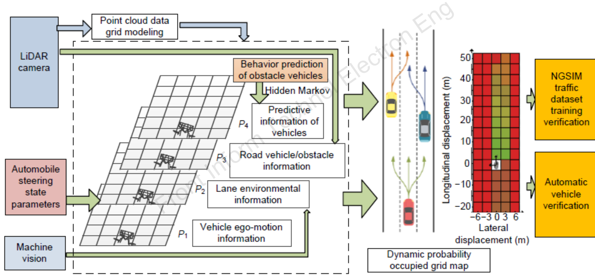
Fig. 2 DGPM algorithm framework
