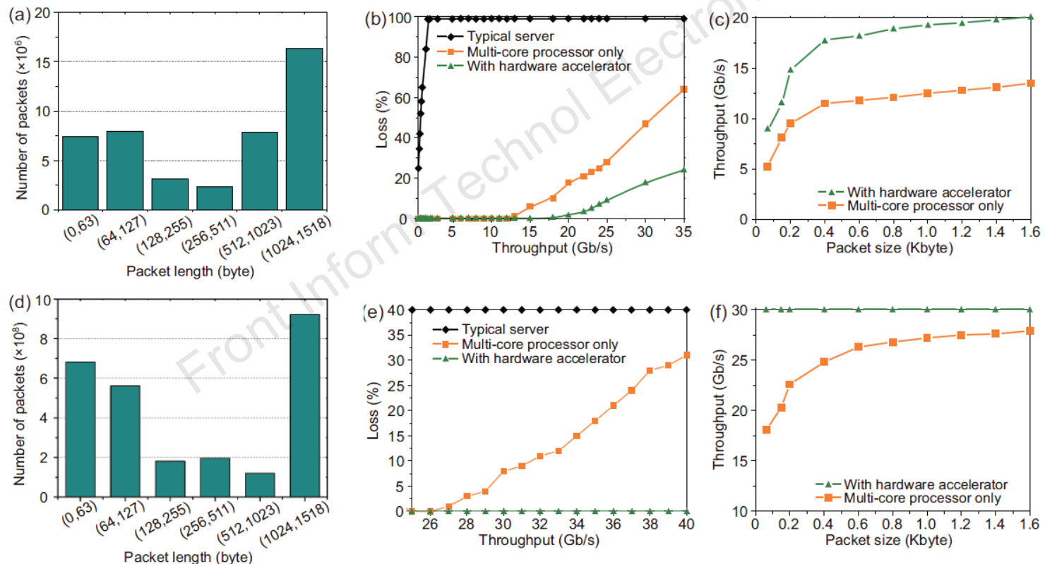
Fig. 12 Results of system performance: (a)–(c) are respectively the packet size distribution, packet loss rate, and throughput in the CDMA2000 core network; (d)–(f) are respectively the packet size distribution, packet loss rate, and throughput in the TD-SCDMA core network
