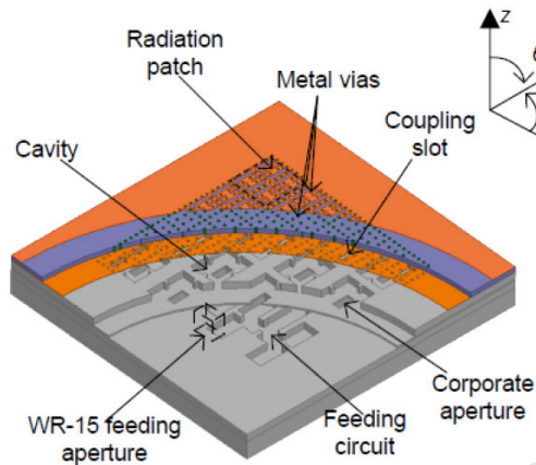
Fig. 1 Linearly polarized antenna array
