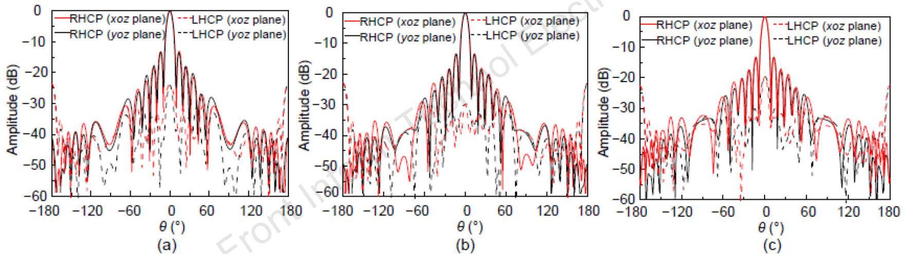
Fig. 31 Simulated radiation patterns of the 8 \times 8 antenna array at 58 GHz (a), 60 GHz (b), and 62 GHz (c) (References to color refer to the online version of this figure)
