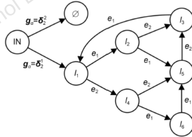
Fig. 3 State transition diagram of A_3
