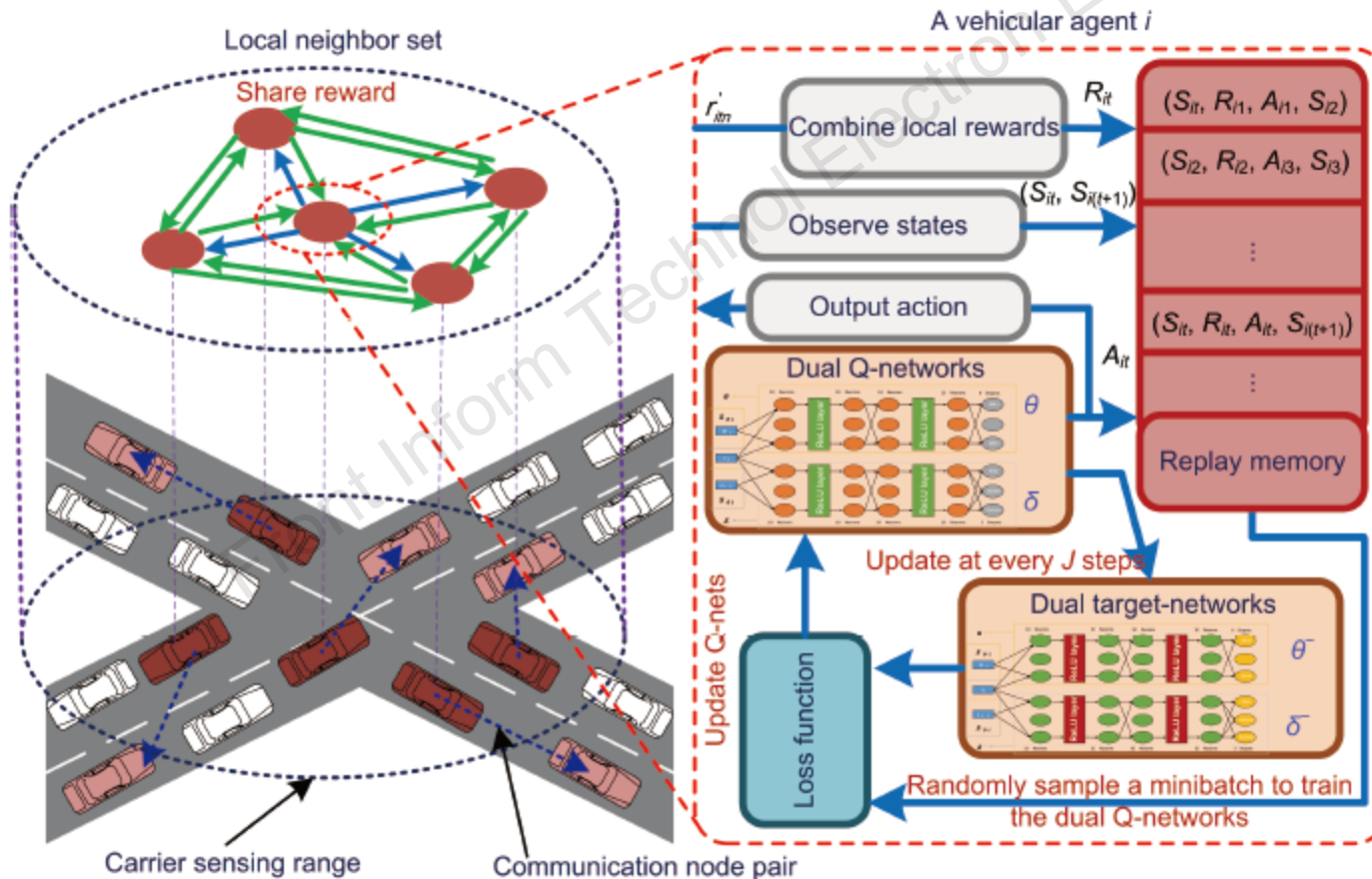
Fig. 2 Scenario of multiple coexisting communication node pairs (CNP) driven by multiagent RL-CDCA
