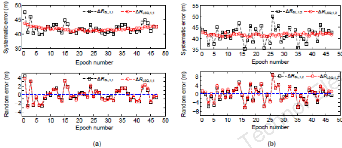
Fig. 7 Error calibration of B1: (a) \varepsilon_{BL,1,1}=1.5 ; (b) \varepsilon_{BL,1,1}=3
