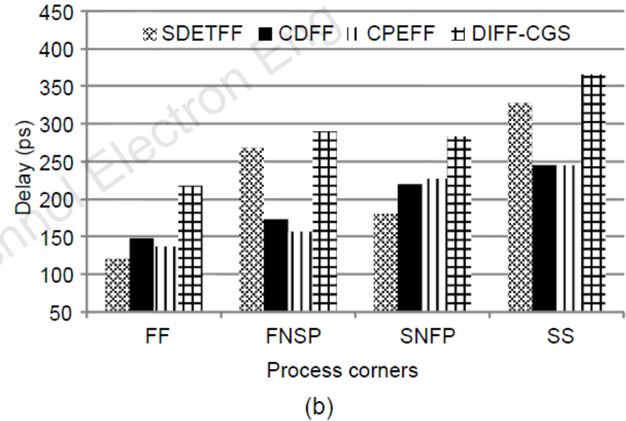
Fig. 13 Different process corners: (a) power dissipation; (b) delay
