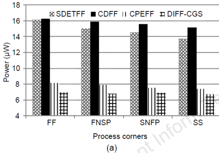
Fig. 13 Different process corners: (a) power dissipation; (b) delay
