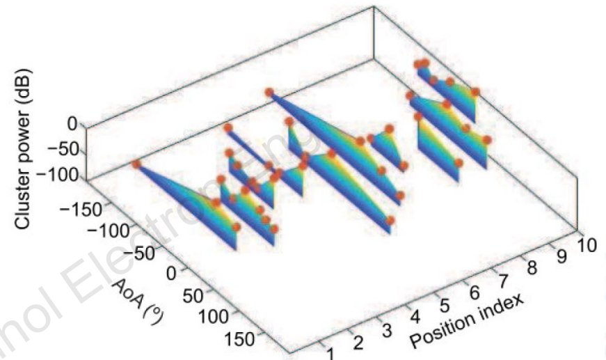
(b) Composite PAS in azimuth of uplink
