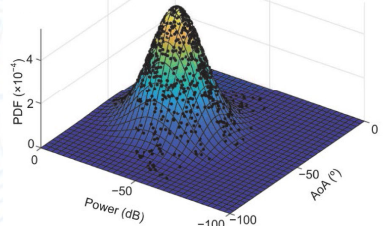
(c) Joint probability density function of rays' AoA and power in downlink
