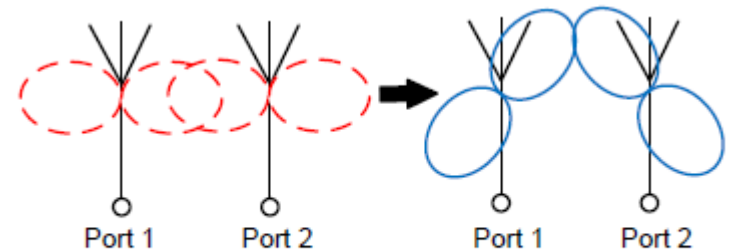
Fig. 8 Schematic of pattern diversity
