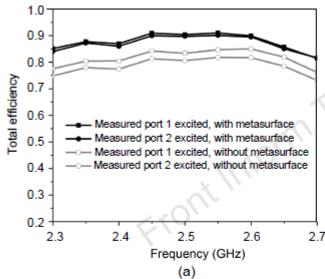
Fig. 18 Total measured efficiency (a) and calculated envelope correlation coefficient (ECC) (b) of two antenna arrays coupled in the H-plane without and with metasurface
