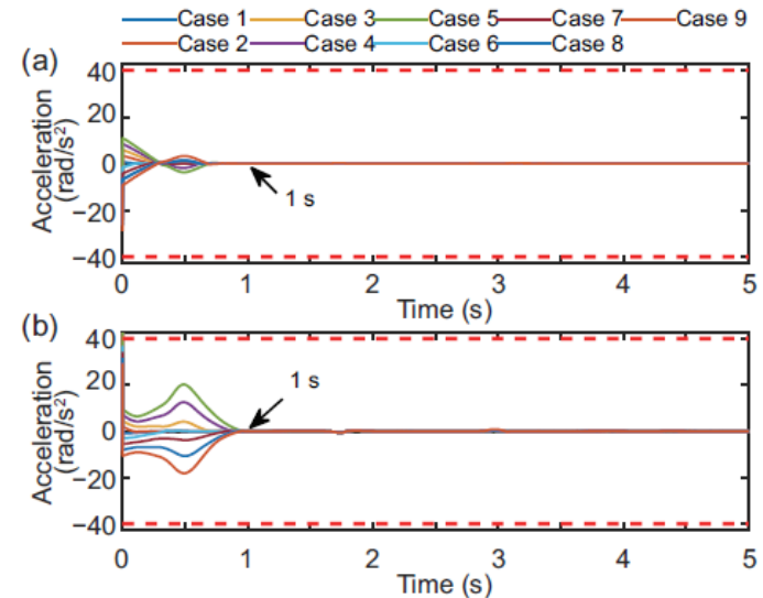
Fig. 7 Acceleration observation errors of \dot{q}_1 (a) and \dot{q}_2 (b)
