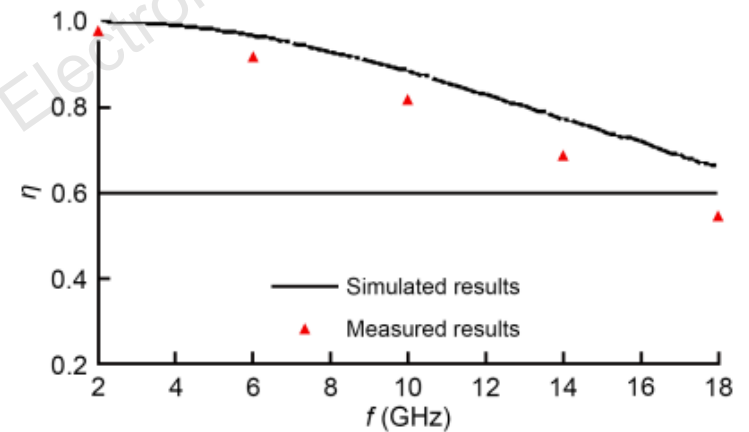
Fig. 9 Measured and simulated power synthesis efficiency
