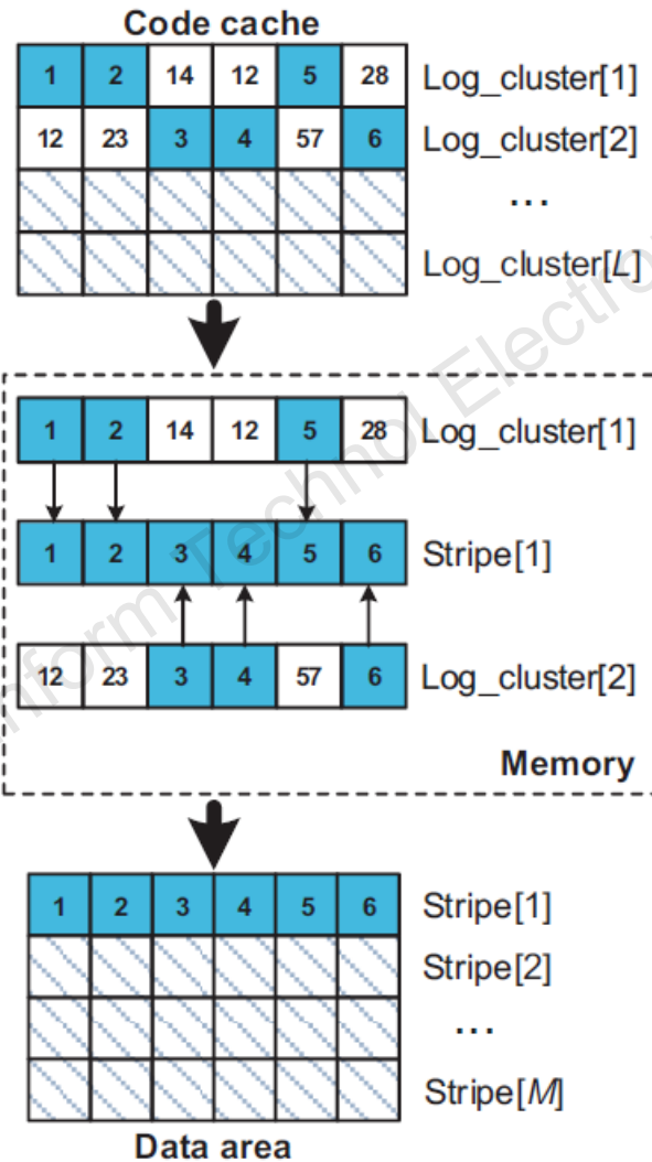
Fig. 4 The destaging process of RERAID
