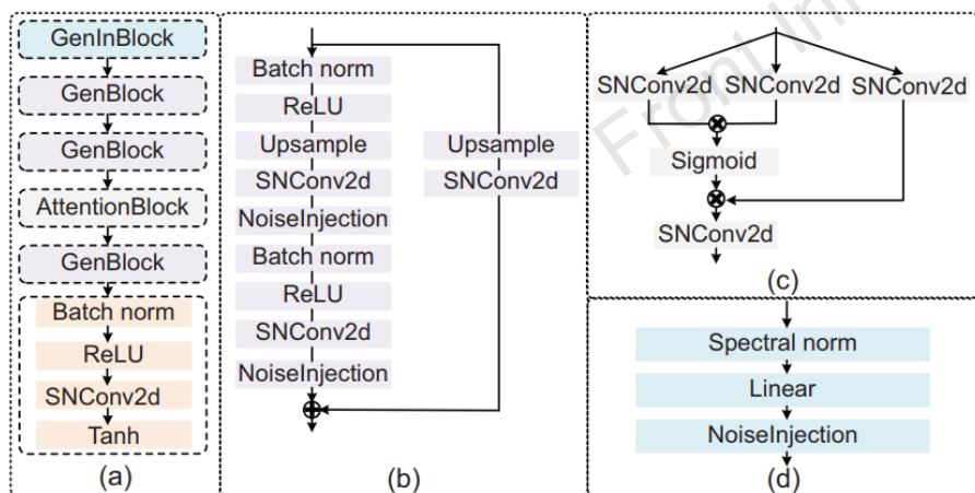
Fig. 4 Details of the generator: (a) generator; (b) \text{GenBlock} ; (c) \text{AttentionBlock} ; (d) \text{GenInBlock}
