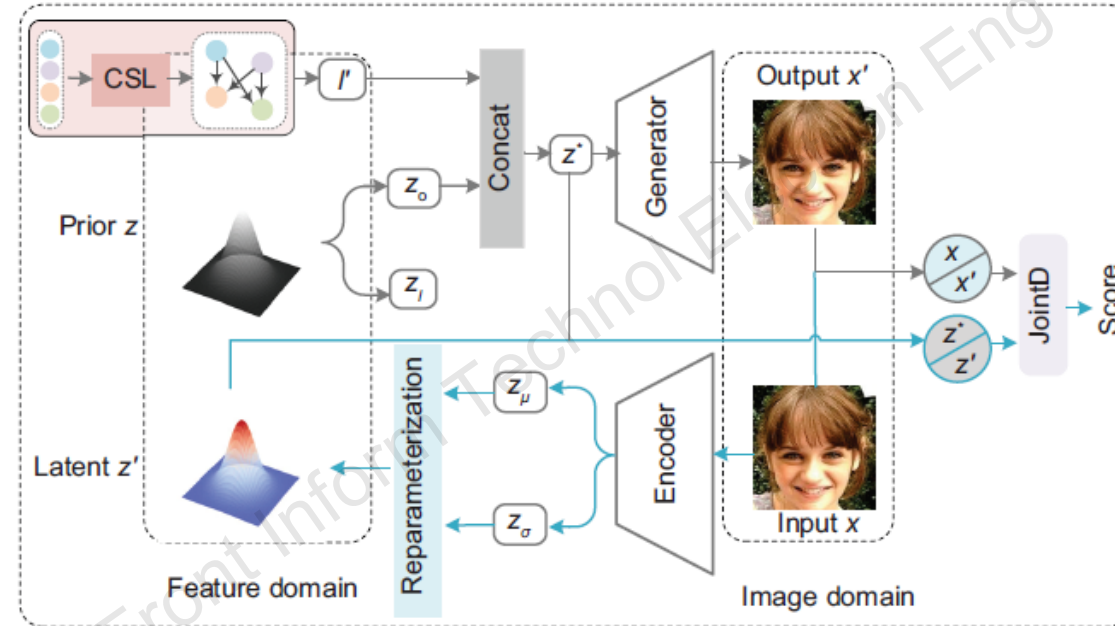
Fig. 1 Overall workflow of our framework. In the training phase, our model first uses the CSL module to learn causality from the image labels, thereby constraining the underlying representation z' = E(x) obtained from the encoder to be consistent with the learned causal relationships. Then, the causal representation l' , which encodes causal relationships between factors of interest in image generation, is used to replace a portion z_l of the prior distribution z , which is then concatenated with the other factors z_o needed for image generation to obtain a new latent representation z^* . This representation is then fed into the generator G to obtain the generated image x' = G(z^*) . Note that JointD is trained alternatively with the generator G and encoder E . In the inference phase, we can achieve causal controllability of an image attribute by modifying the value of a latent representation along a specific dimension, i.e., causal intervention
