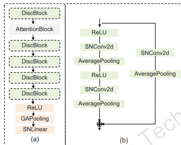
Fig. 5 Detail of discriminator D_x : (a) discriminator; (b) \text{DiscBlock}
