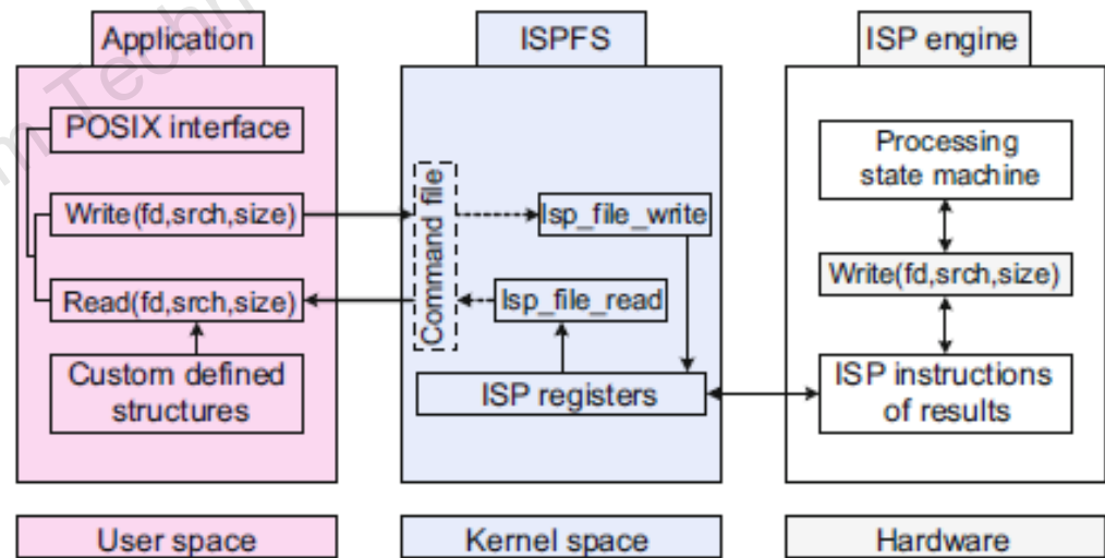
Fig. 3 In-storage processing mechanism
