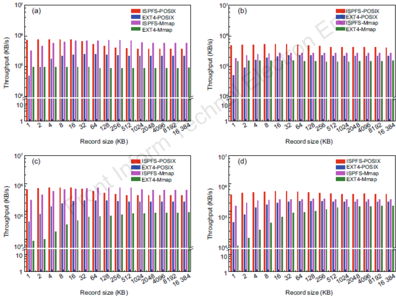
Fig. 7 Comparing throughput for ISPFSS using IOZONE: (a) rewrite; (b) reread; (c) random write; (d) random read
