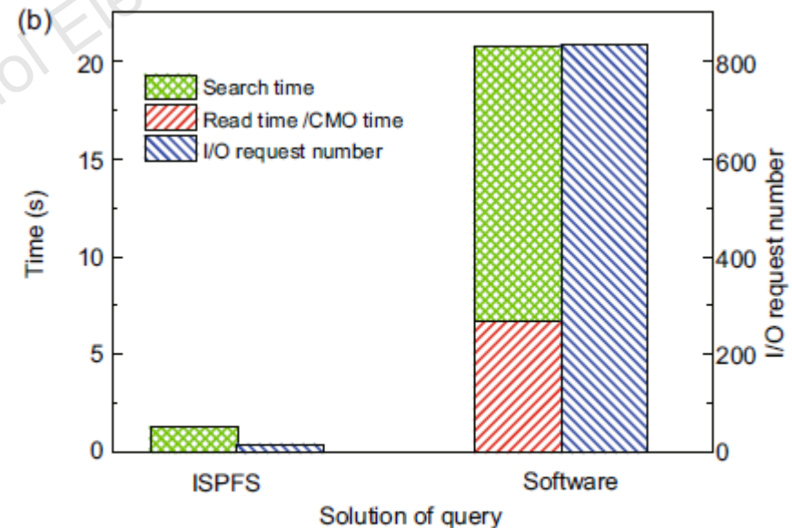
Fig. 9 The resource usage (a) and access time and I/O requests (b)
