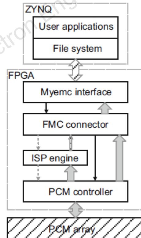
Fig. 1 Architecture of the proposed storage system
