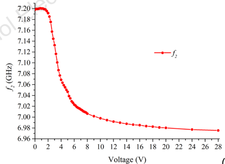
Fig. 5 Experimental results of the resonant frequency as a function of the applied voltage: (a) low resonant frequency f_1 ; (b) high resonant frequency f_2
