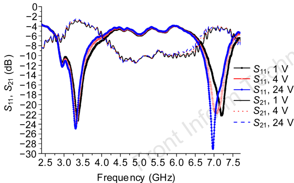
Fig. 4 Experimental results of S_{11} and S_{21} spectra of SIR when the applied voltage is 1, 4, or 24 V
