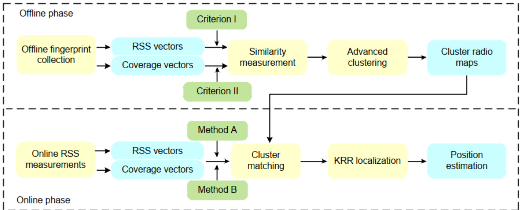
Fig. 1 The proposed indoor positioning algorithm
