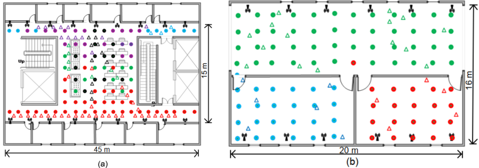
Fig. 2 Layouts of the experimental sites: (a) LA; (b) LB Each dot denotes one RP, and different colors for the RPs indicate different clusters. Each triangle represents the location of each online test point with the corresponding cluster.
