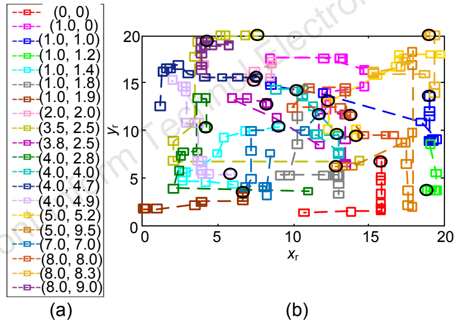
Fig. 11 The selected start points in \text{Set}(x_{r,0}, y_{r,0}) (a) and the corresponding start point group in \text{Set}(x'_{r,0}, y'_{r,0}) (b)
