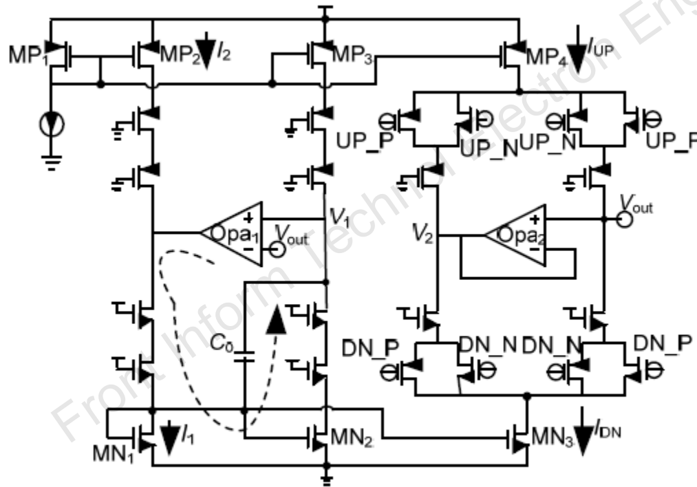
Fig. 7 The proposed CP topology
