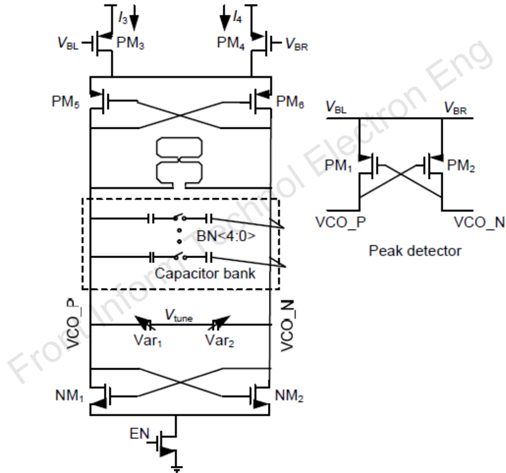
Fig. 1 The proposed voltage-controlled oscillator (VCO) with an automatic amplitude control (AAC) circuit and a figure-8-shaped inductor
