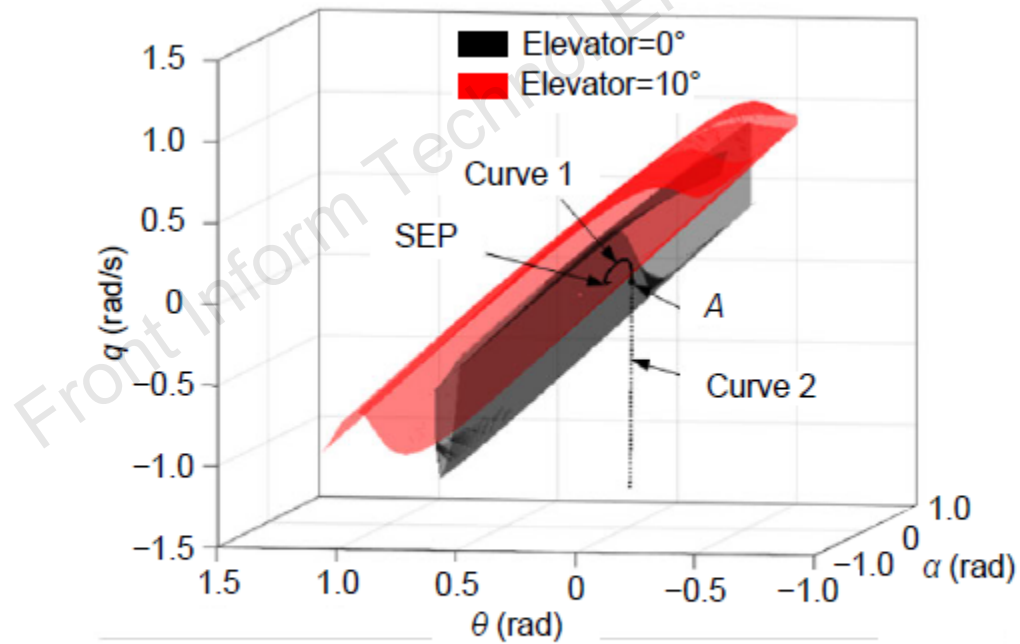
Fig. 7 Change of envelope with the pilot operation References to color refer to the online version of this figure
