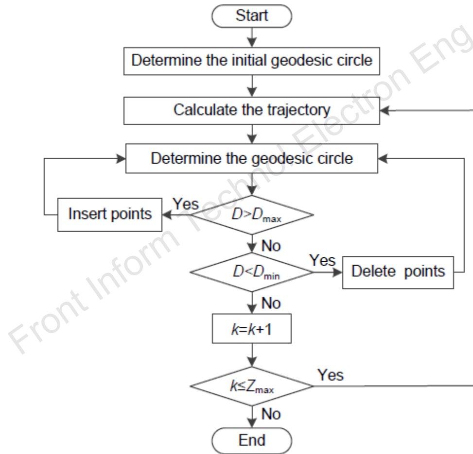
Fig. 1 Flow chart of envelope determination in the geodesic circles method
